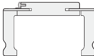
Profilzarge PZ 2
